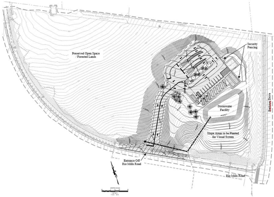
Figure 5 – Northern Convenience Center Site Plan
