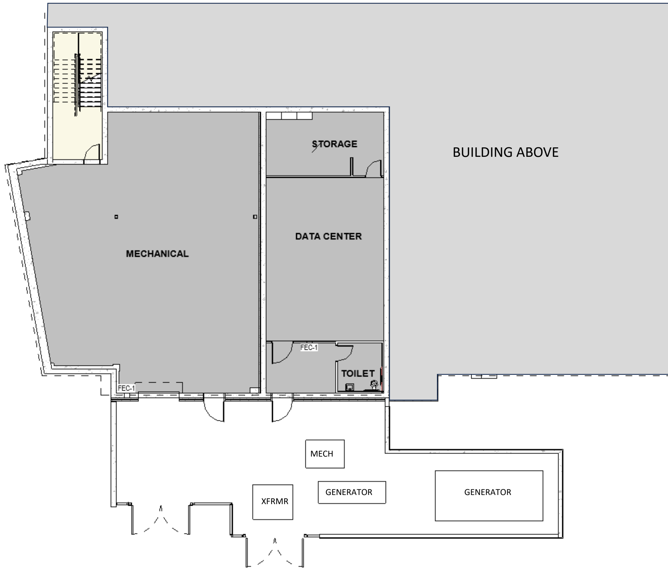
Basement Level Floor Plan – Equipment Yard
