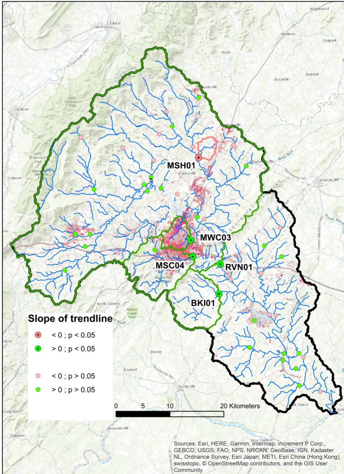
Figure 2. Rivanna Watershed and benthic sampling sites. Sites are distinguished based on the slope direction (negative slope (<math>< 0</math>) = red; positive slope (> 0) = green) and the significance of the trend (larger circle with center dot = significant; smaller circle = insignificant). The background image is impervious coverage for 2016.
